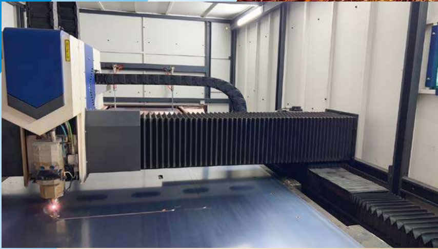
雷射導光罩 Laser Bellows Cover
